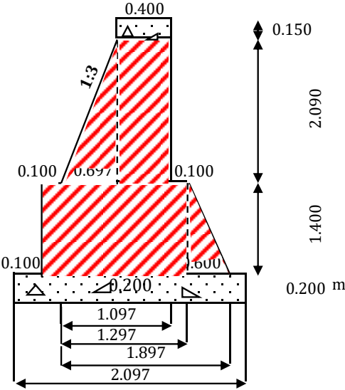
Section of Return Wall
