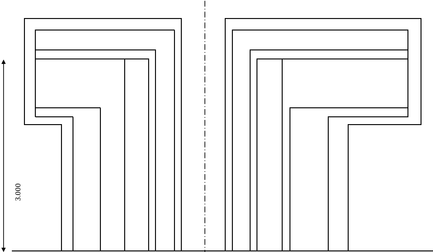
HALF PLAN
