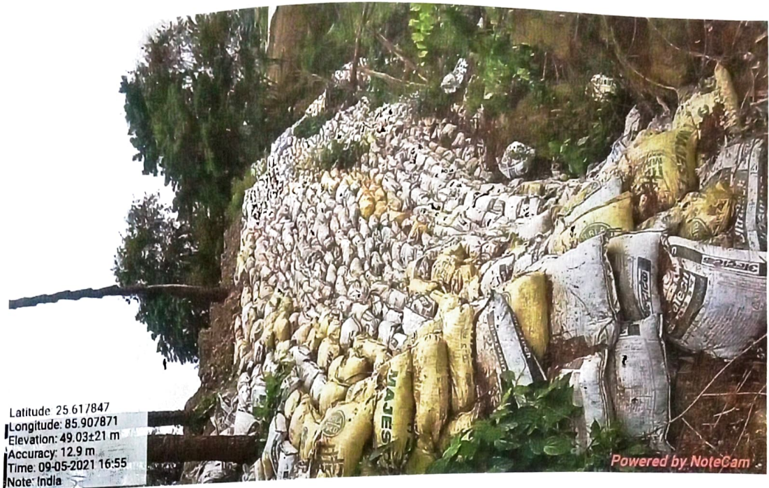
General View of Repaired Road
